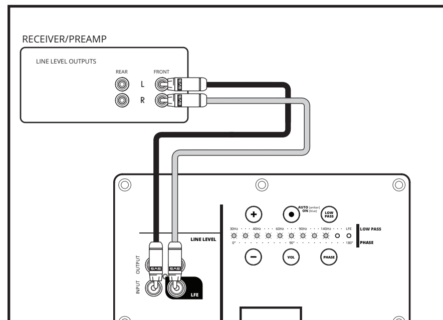
Line Level Connection – Stereo Receiver or Preamp Left/Right Channels
